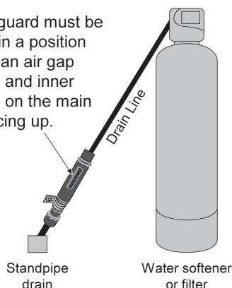
Mounting option 1
